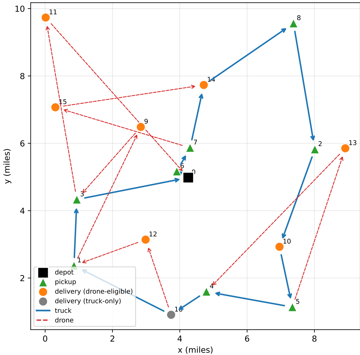
V6 DAPDP optimum (16.10.3) z = \$3.011
